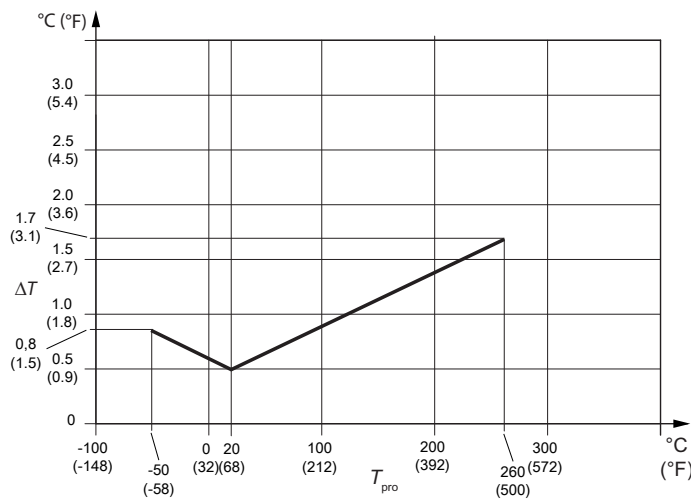
Fig. 10: Temperature accuracy
