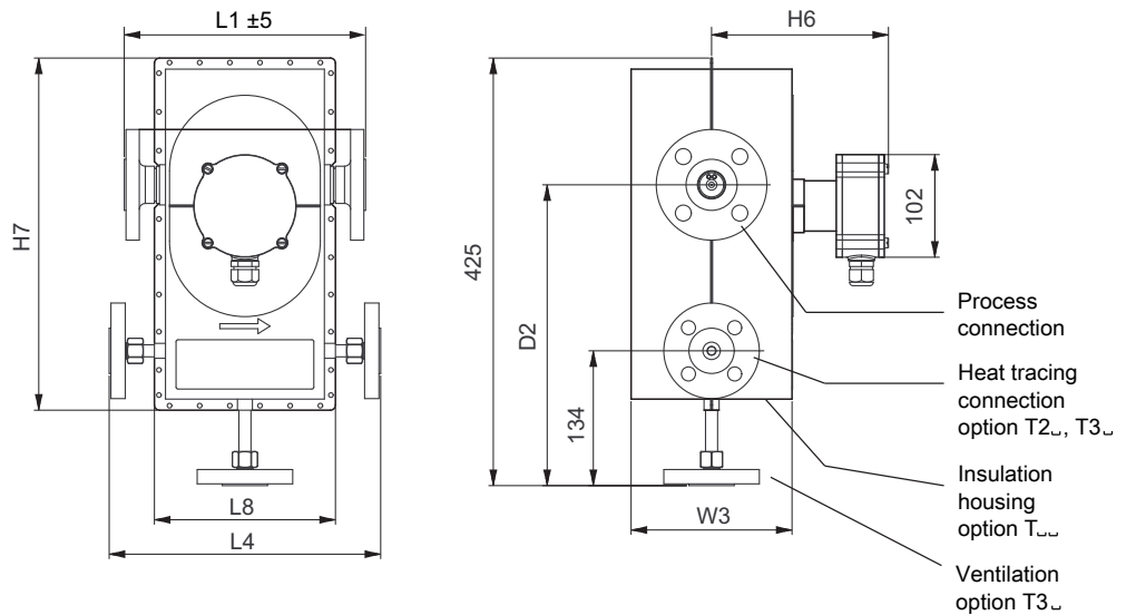
Fig. 27: Dimensions in mm: version with insulation housing
