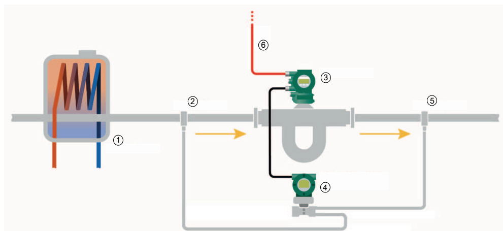
Fig. 52: Positioning of pressure taps
