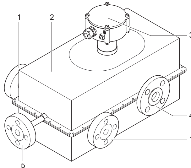
Fig. 21: Configuration of Rotamass with insulation and heat tracing
