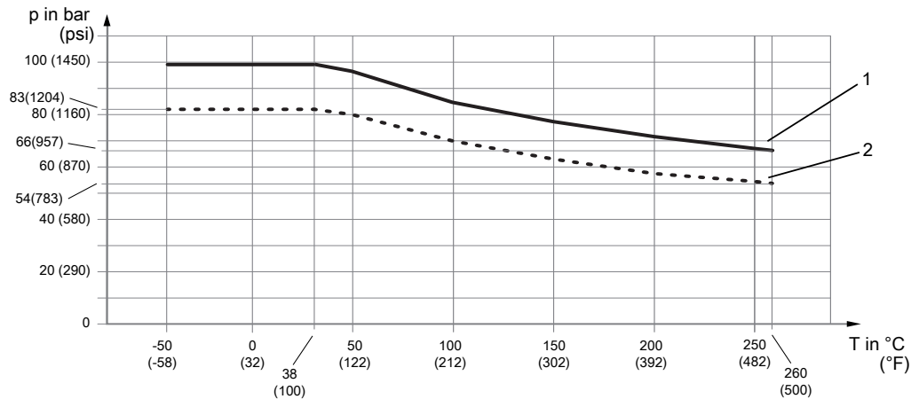
Fig. 14: Allowed process pressure as a function of process connection temperature
