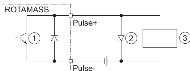
Fig. 49: Passive pulse output connection with electromechanical counter
