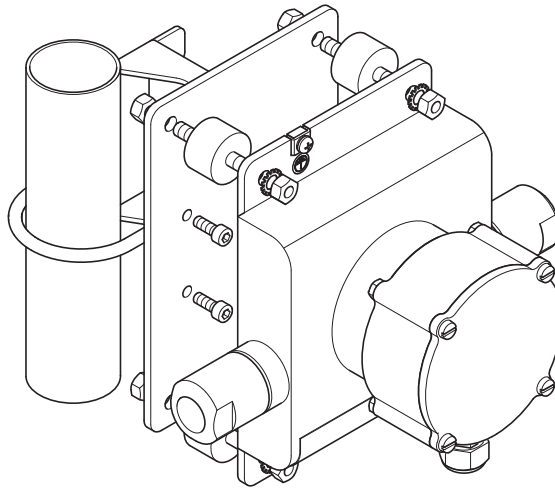
Fig. 53: Fixing device option PD for Rotamass Nano sensor
