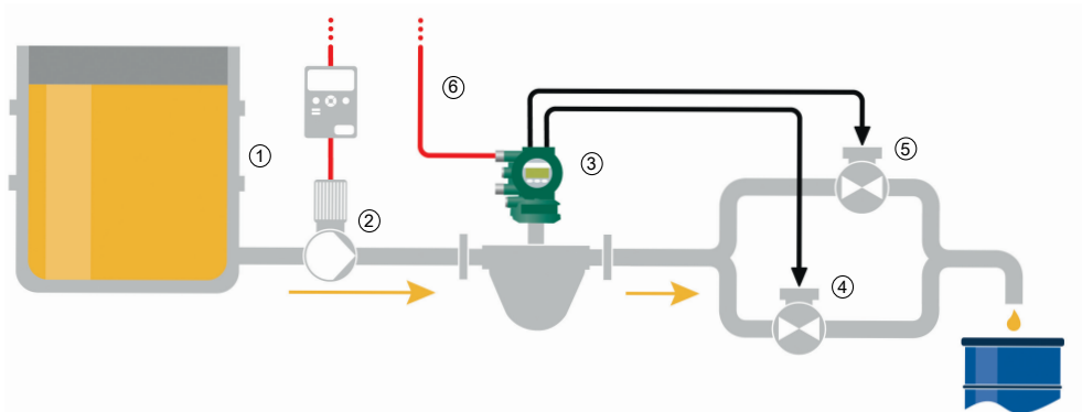
Fig. 51: Two-stage mode (The above diagram illustrates the fundamental functionality for one of several combination possibilities)
