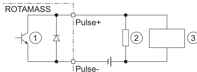
Fig. 48: Passive pulse output connection with electronic counter
