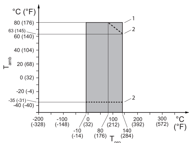
Fig. 23: Allowed process fluid and ambient temperatures, remote type for process connection type HS4 and HS8
