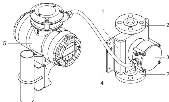
Fig. 5: Configuration of the Rotamass remote type
