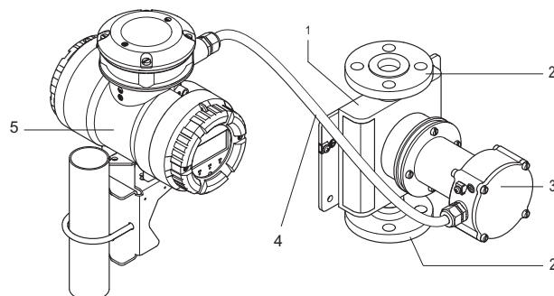
Fig. 6: Configuration of the Rotamass remote type - long neck
