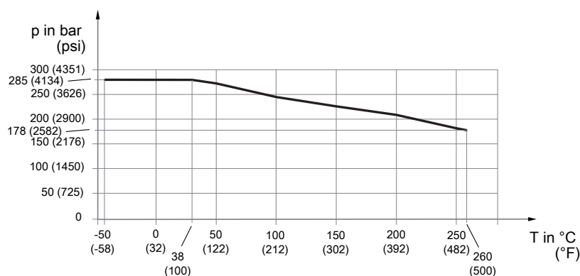
Fig. 20: Allowed process pressure as a function of process connection temperature
